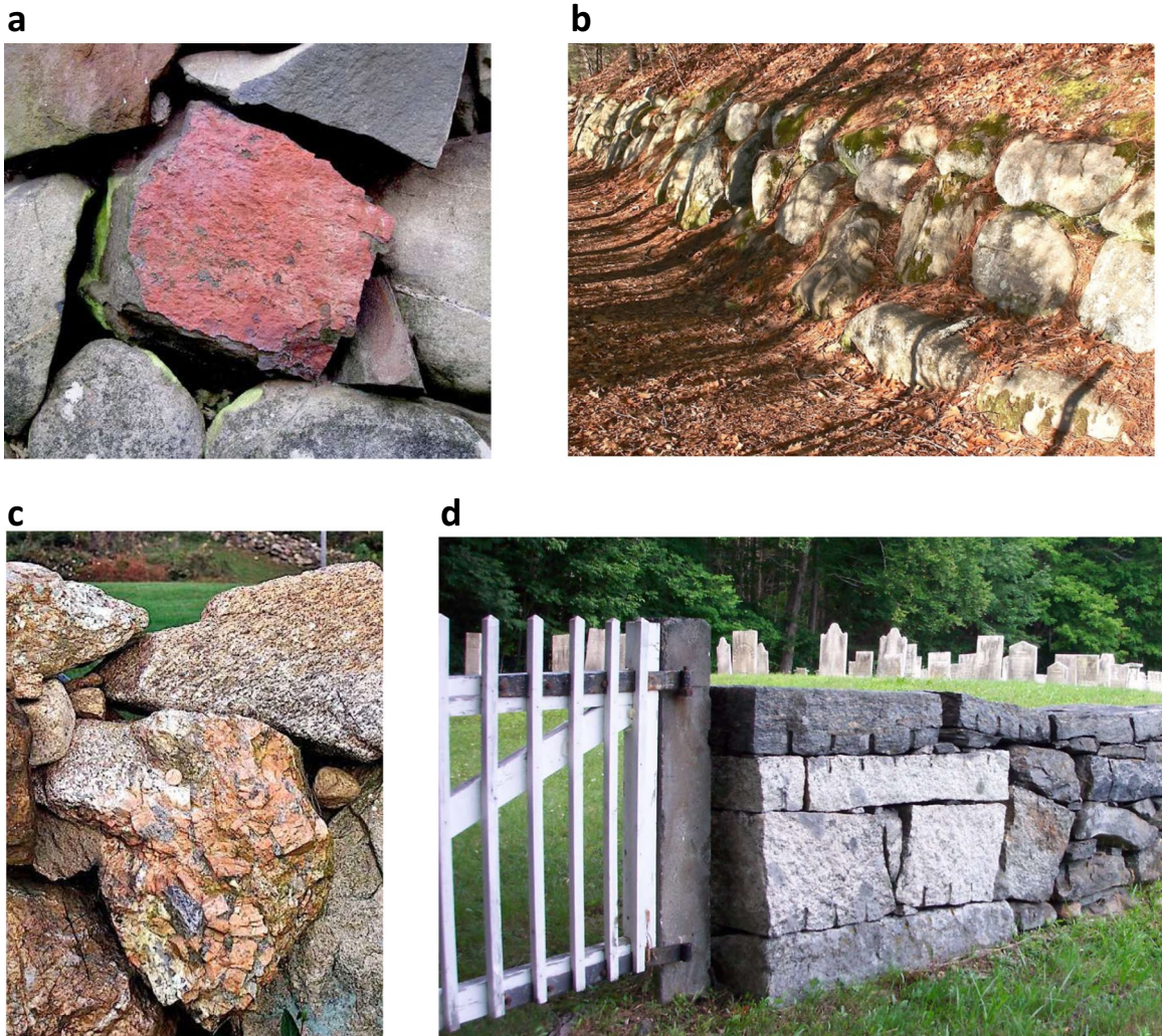
Fig. 6 Examples of contrasting materials and sources. (a) Laid single wall in Farmington, Connecticut, built of angular basalt traprock talus at top and rounded gneiss boulders at base. The central stone is coated with red jasper as a hydrothermal precipitate. (b) Pitstone (from gravel pit) of granite laid in normal ( Subtype ), retaining ( Type ), flanking ( Family ) wall ( Class ) in Concord, Mas-
