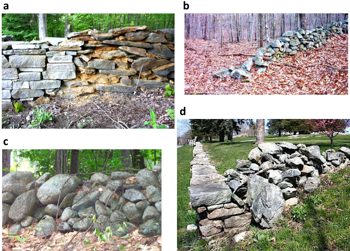
Fig. 8 Examples of contrasting terminations (ends of walls) and contacts (ends of wall segments). (a) Segment of laid double wall of quarried granite slabs was built against a disintegrating segment of single wall dominated by quarried (pyrrhotite-bearing) schist. By definition, this one wall has two abutting segments with a non-vertical contact. (b) Unbuilt tip of final segment of single wall is a termination. (c) Wall in
